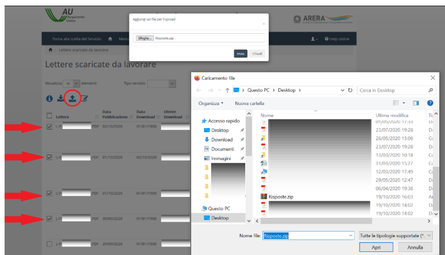
Fig. 7 Upload multipli
